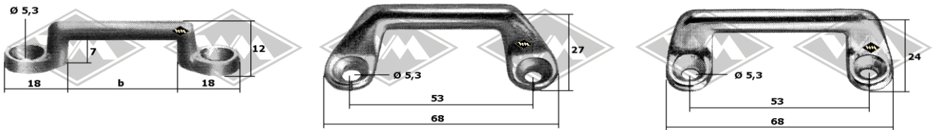
Lakai-Krampe vernickelt M51 b = 25 mm
